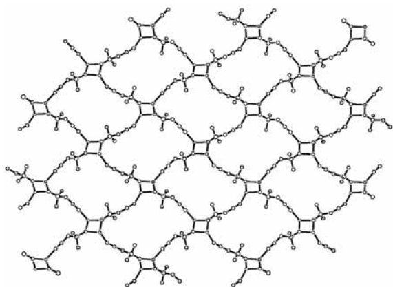
Fig. 5 Polymeric sheet network for compound 2 with all hydrogen atoms, THF molecules and carbons of the \text{Pr}^1 groups removed for clarity.
